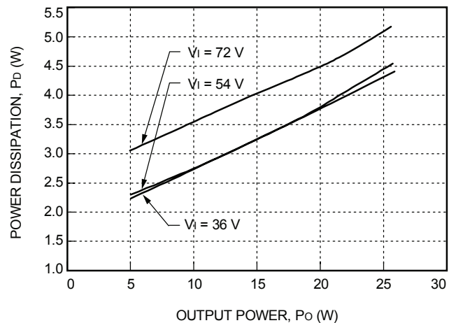
Figure 23. DW025ABK-M Fixed Losses, P_P
