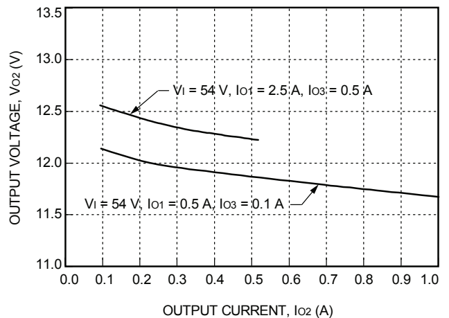
Figure 5. DW025ABK-M Typical Load Regulation
