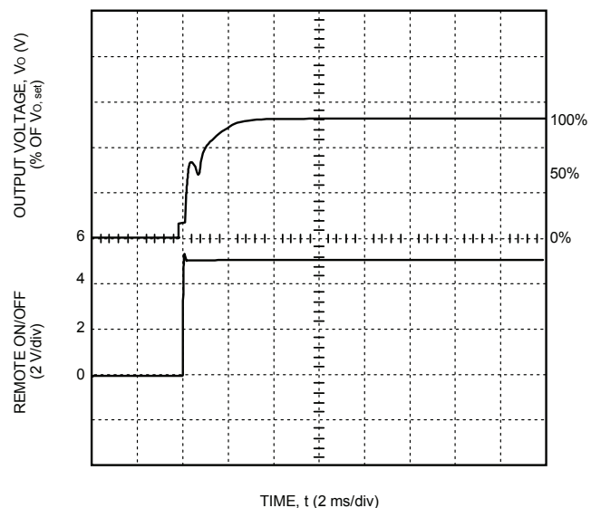
Figure 17. DW025 Triple Output-Series Typical Output Voltage Start-Up when Signal Applied to Remote On/Off
