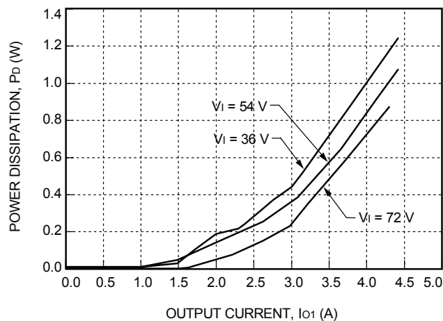
Figure 25. DW025ABK-M, DW025ACL-M Losses, Associated with 5 V Output, P_{s1}
