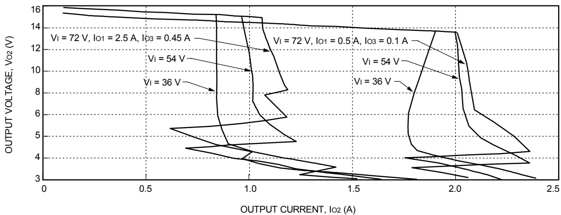
Figure 12. DW025ACL-M Typical 15 V Output Characteristics
