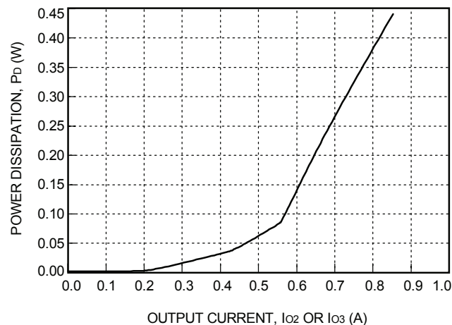
Figure 27. DW025ACL-M Losses Associated with \pm 15 V Output, P_{s2}/P_{s3}
