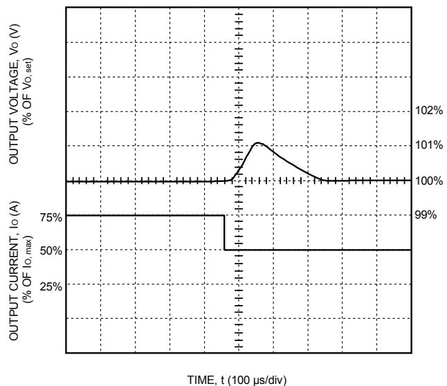
Figure 15. DW025 Triple Output-Series Typical Output Voltage for a Step Load Change from 75% to 50% of Full Load on Output 1
