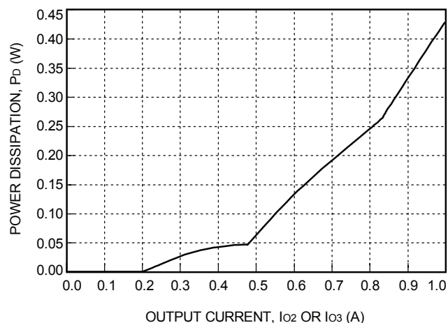
Figure 26. DW025ABK-M, Losses Associated with \pm 12 V Output, P_{s2}/P_{s3}
