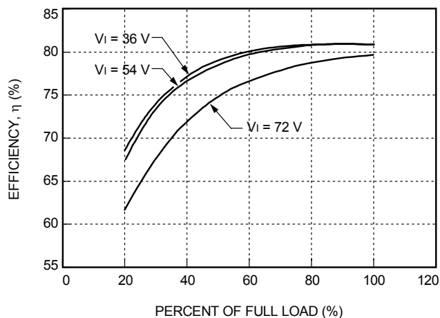
Figure 14. DW025ACL-M Typical Converter Efficiency
