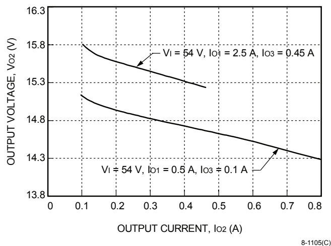
Figure 7. DW025ACL-M Typical Load Regulation
