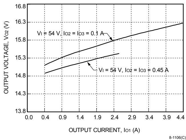
Figure 8. DW025ACL-M Typical Cross Regulation with Respect to I_{01}
