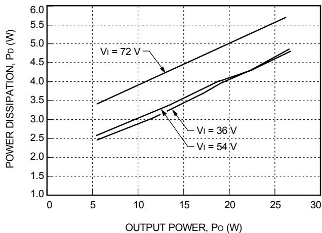
Figure 24. DW025ACL-M Fixed Losses, P_p
