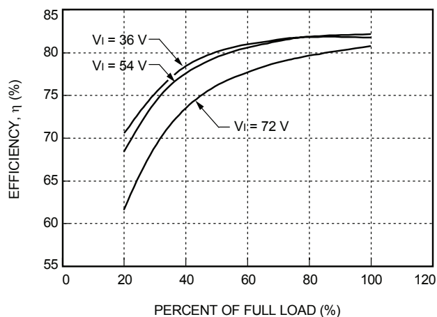
Figure 13. DW025ABK-M Typical Converter Efficiency
