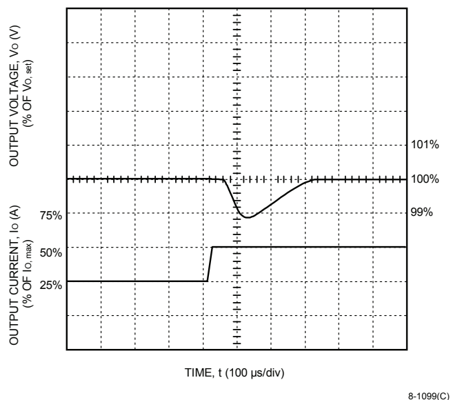
Figure 16. DW025 Triple Output-Series Typical Output Voltage for a Step Load Change from 25% to 50% of Full Load on Output 1
