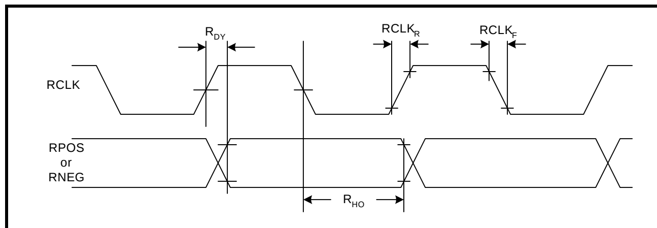
FIGURE 29. RECEIVE CLOCK AND OUTPUT DATA TIMING
