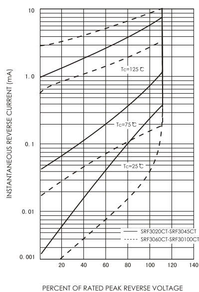
FIG.4-TYPICAL REVERSE CHARACTERISTICS
