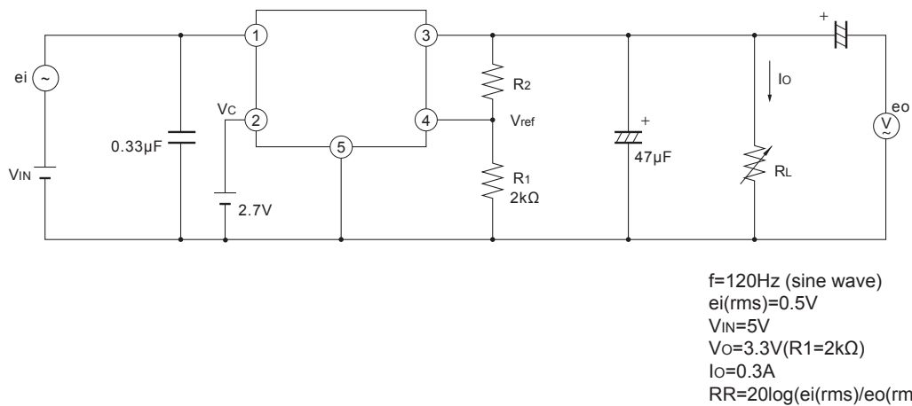
Fig.2 Test Circuit for Ripple Rejection
