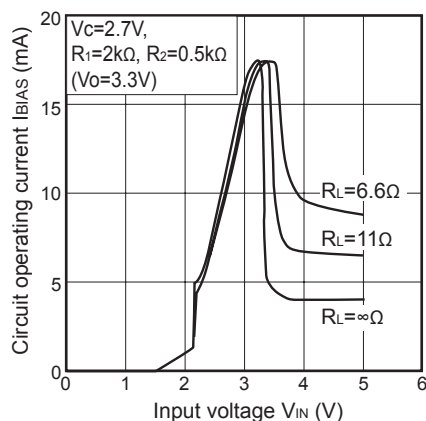
Fig.16 Circuit Operating Current vs. Input Voltage (PQ20WZ51J00H)
