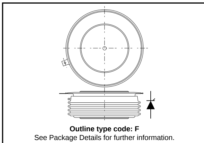
Fig. 1 Package outline
