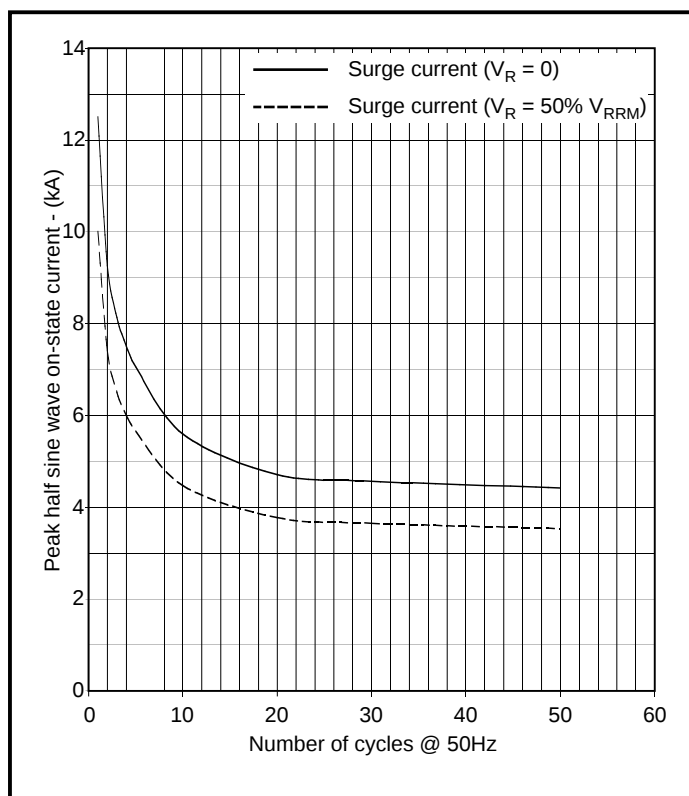
Fig.8 Multi-cycle surge currents
