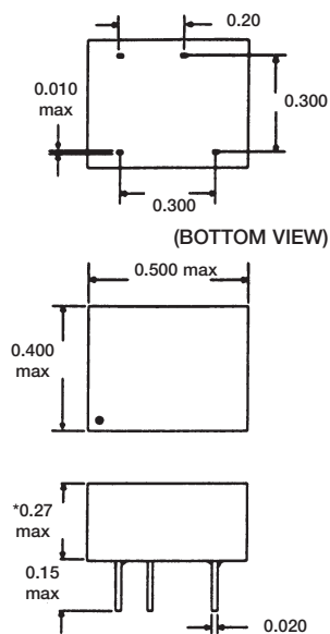
DUAL-IN-LINE PACKAGE
