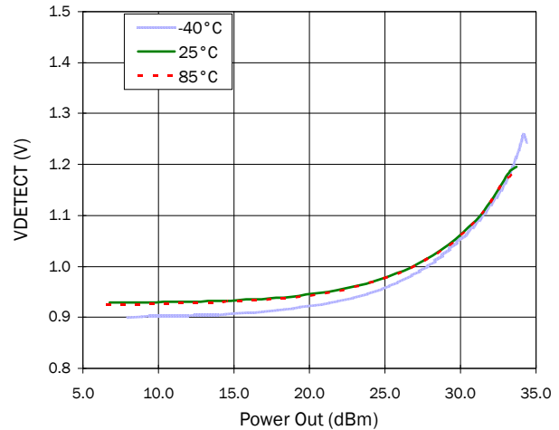
VDETECT versus Output Power @1960MHz
