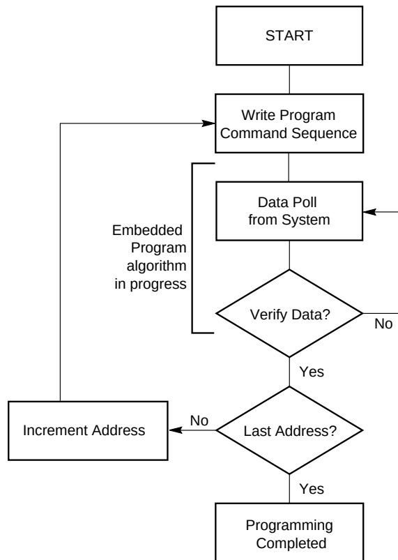
Figure 4. Program Operation
