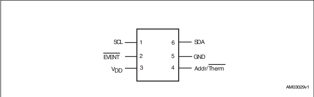
Figure 2. Pinout
