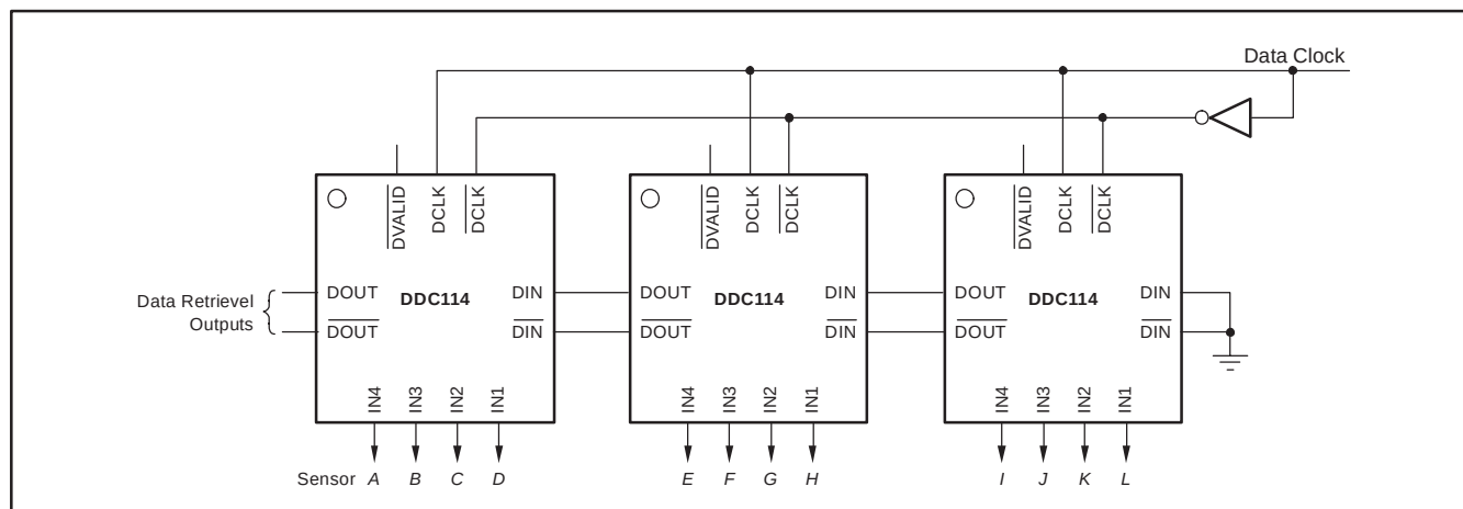
Figure 21. Daisy-Chained DDC114s
