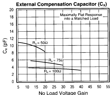
Figure 6: External Compensation Capacitance ( C_x )
