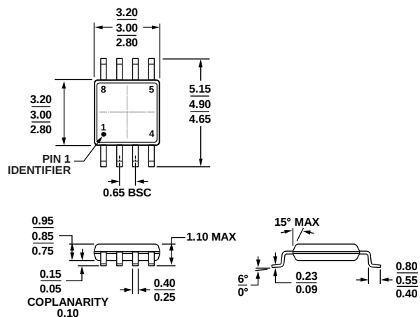
COMPLIANT TO JEDEC STANDARDS MO-187-AA Figure 8. 8-Lead Mini Small Outline Package [MSOP] (RM-8)
