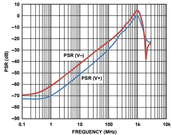
Figure 32. ADV3220 PSR
