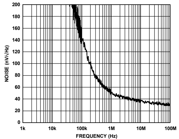
Figure 33. ADV3220 Noise vs. Frequency
