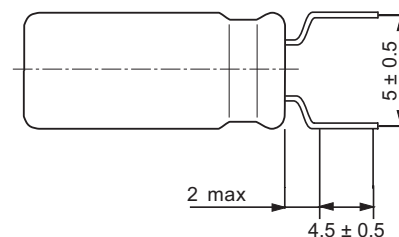
5 \leq \text{ØD} \leq 8 Leads bent open, shortened EKS 09... (S = 5 mm)
