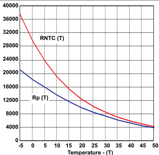
Figure 48. NTC [R(T)] and NTC in Parallel to RT2 [Rges(T)]
