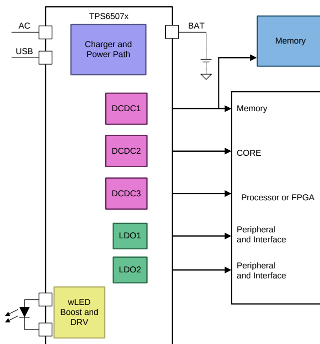
Block Diagram
