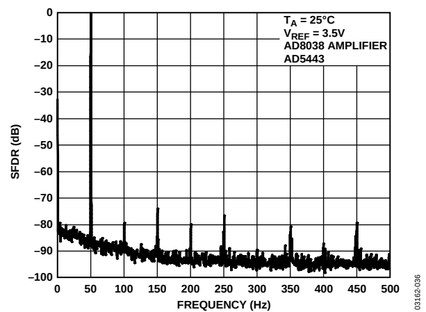
图35. 宽带SFDR f_{OUT} = 50\text{ kHz} , 更新速率 = 1 MHz
