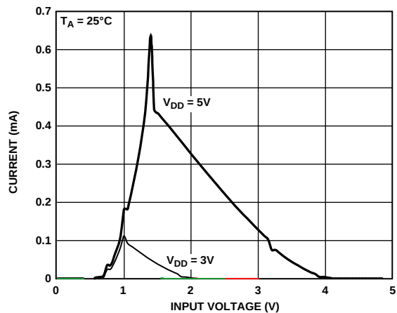
图21. 电源电流与逻辑输入电压的关系, \overline{SYNC}(SCLK) , DATA = 0
