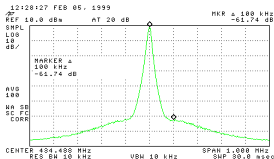
3.5V Phase Noise MODIN=3k
