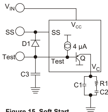
Figure 15. Soft Start
