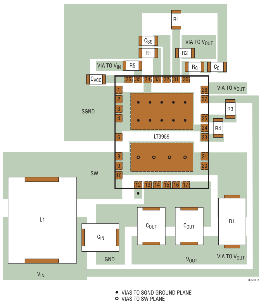
Figure 5. Suggested Layout of the 2.5V to 8V Input, 12V Output Boost Converter in the Typical Application Section
