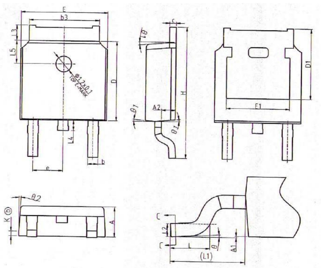
COMMON DIMENSIONS
