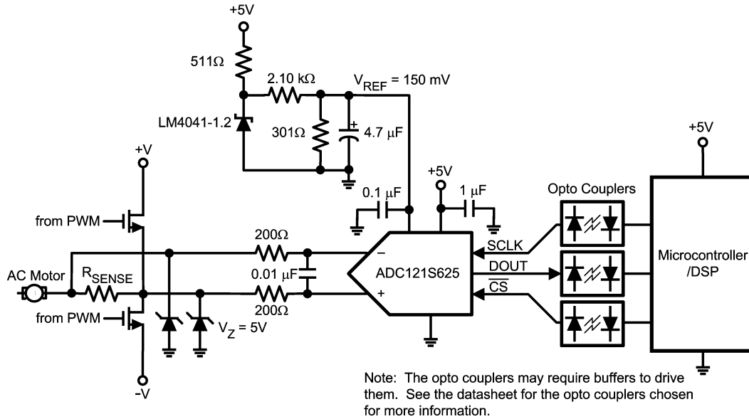
FIGURE 4. Motor Control using isolated ADC121S625
