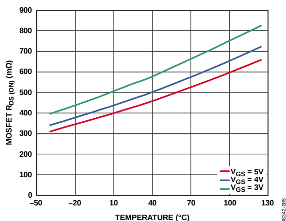
Figure 23. MOSFET R_{\text{DS(ON)}} vs. Temperature (Pin-to-Pin Measurements)
