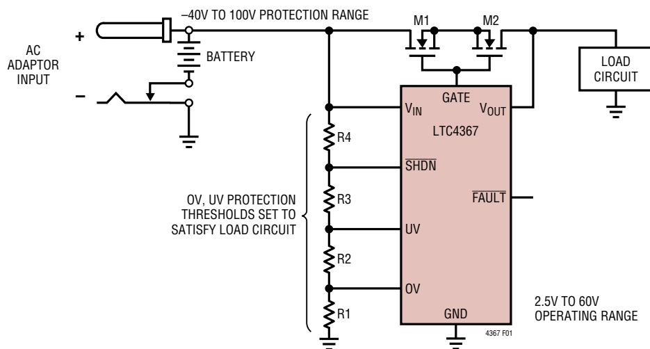
Figure 1. Polarity Protection for DC Barrel Connectors
