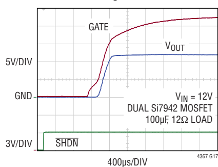
Turn-On Timing
