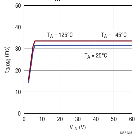
LTC4367 GATE Turn-On Delay Time vs V_IN
