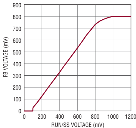
RUN/SS vs FB Voltage
