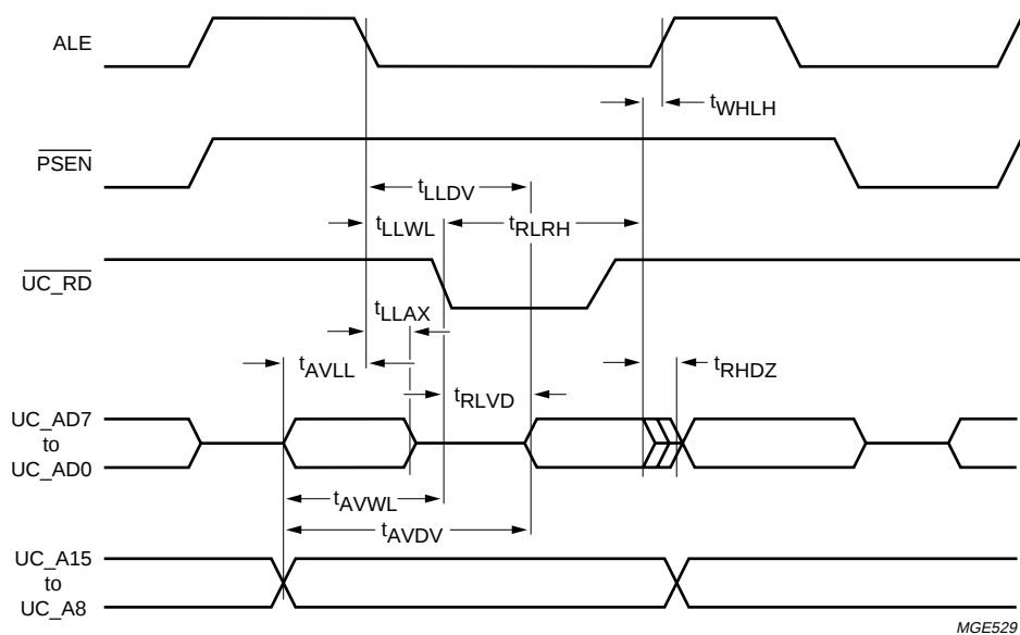
Fig.27 External data memory read cycle.
