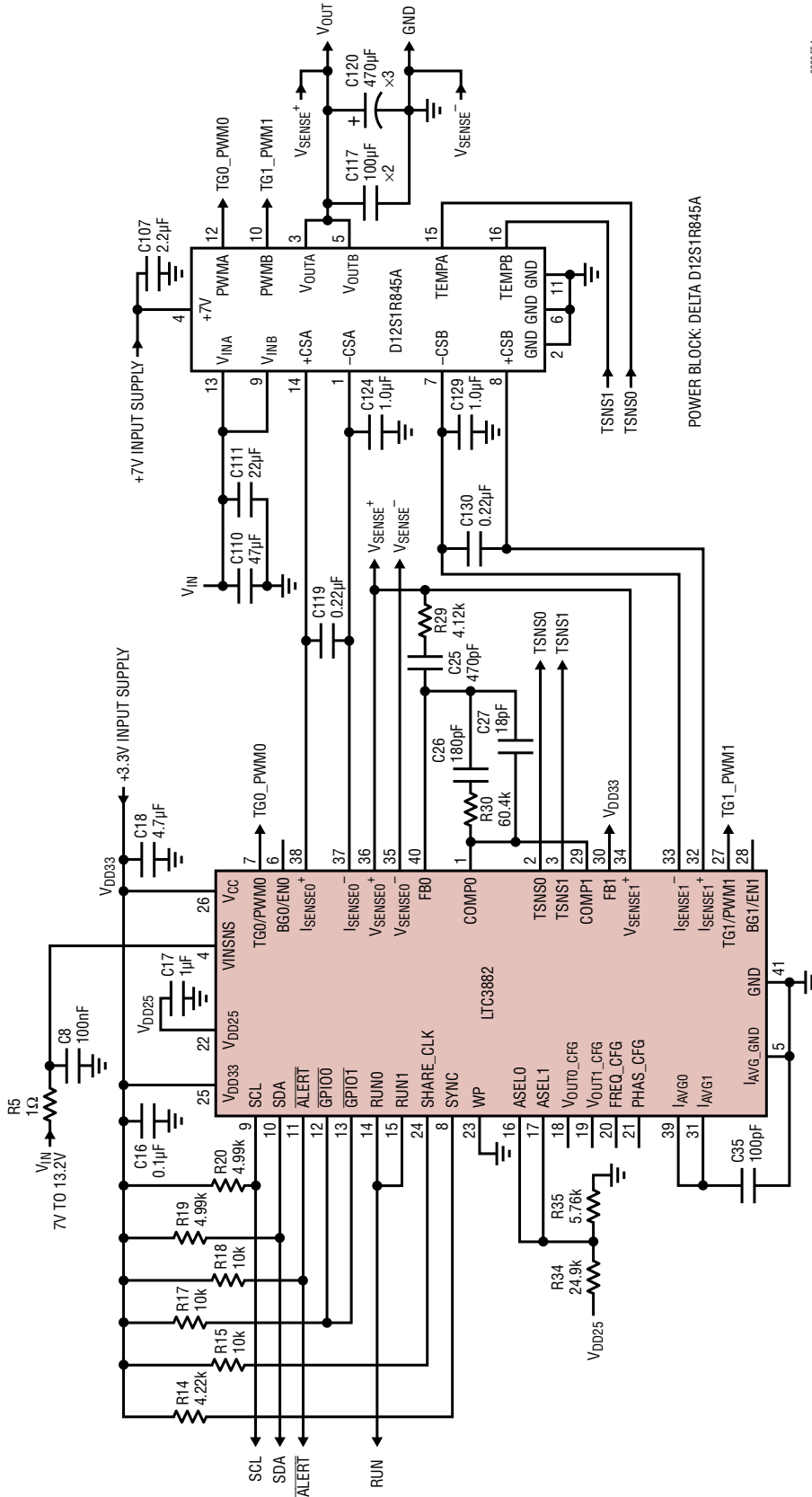
Figure 54. High Density 1.5V/45A 650kHz Converter Using Dual Power Block
