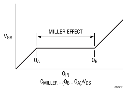
Figure 21. Typical MOSFET Gate Charge Curve
