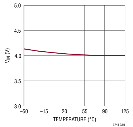
Internal UVLO
