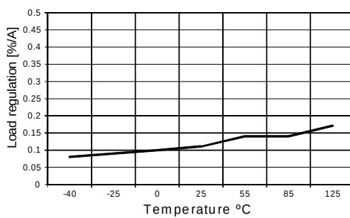
Figure 16: Load regulation vs temperature ( V_{in} = 1.5\text{ V} , 0 < I_{out} < 2\text{ A} )
