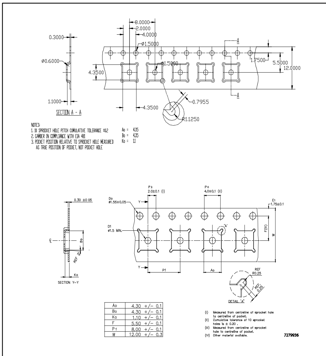
Figure 34: DFN8 (4 x 4 mm) tape (all dimensions are in mm)
