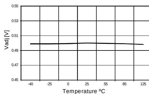
Figure 11: Reference voltage vs temperature ( V_{in} = 1.5\text{ V} , I_{out} = 10\text{ mA} )
