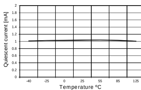
Figure 13: Quiescent current vs temperature ( V_{in} = 1.5\text{ V} , I_{out} = 2\text{ A} )
