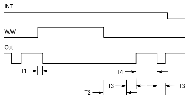
Figure 4. Switching Waveform W/W and INT Active
