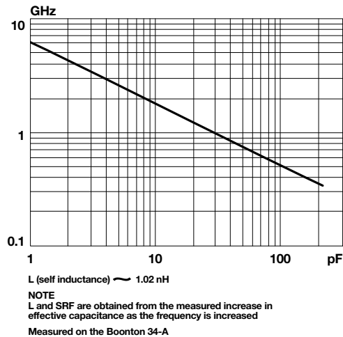
Typical Self Resonant Frequency vs. Capacitance Accu-P® 1210
