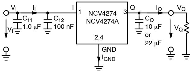
Figure 2. Measuring Circuit
