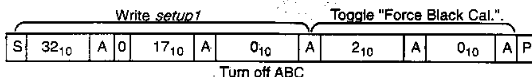
Figure 19 : Same location multiple data write.
