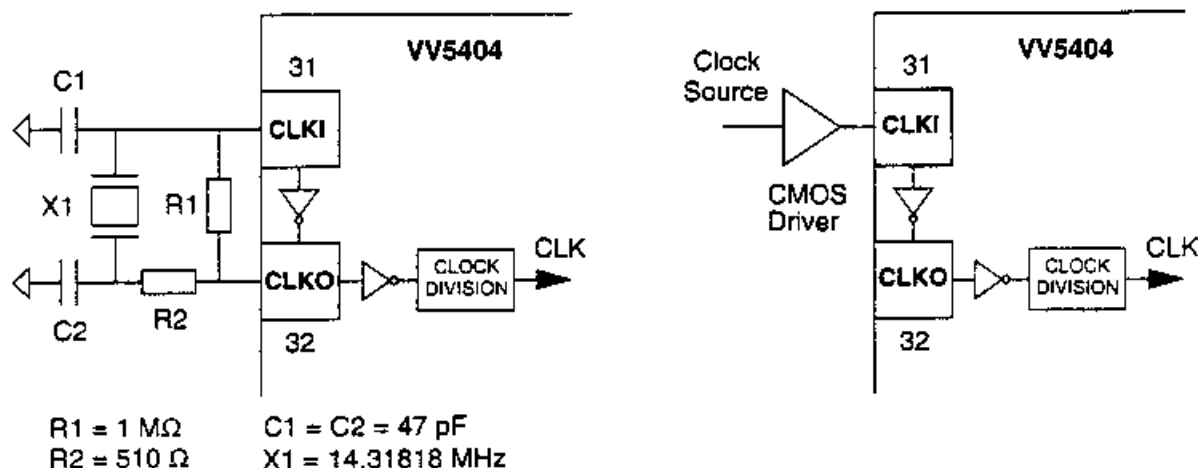
Figure 24 : Camera Clock Sources
