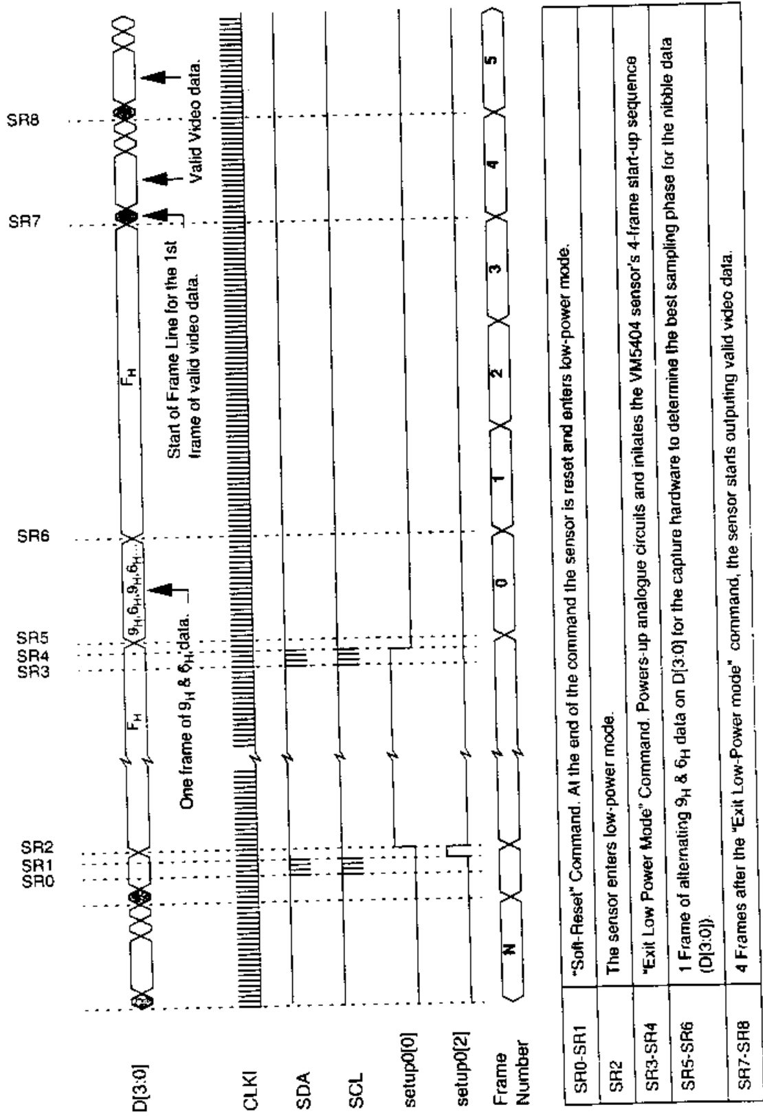
Figure 7 : Resetting the VV5404 Sensor via the Serial Interface.
