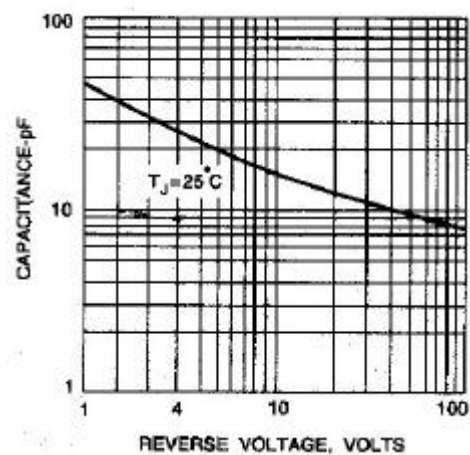
Fig. 4-TYPICAL JUNCTION CAPACITANCE
