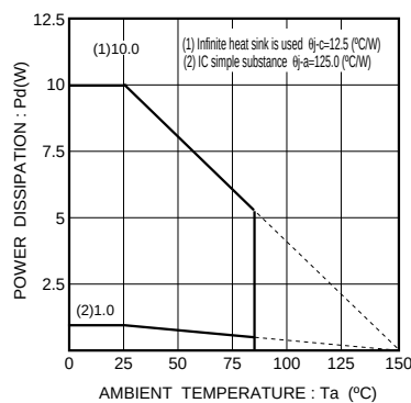
Fig.8 Thermal derating curves (TO252-5)
