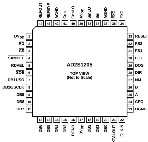
Figure 2. Pin Configuration
