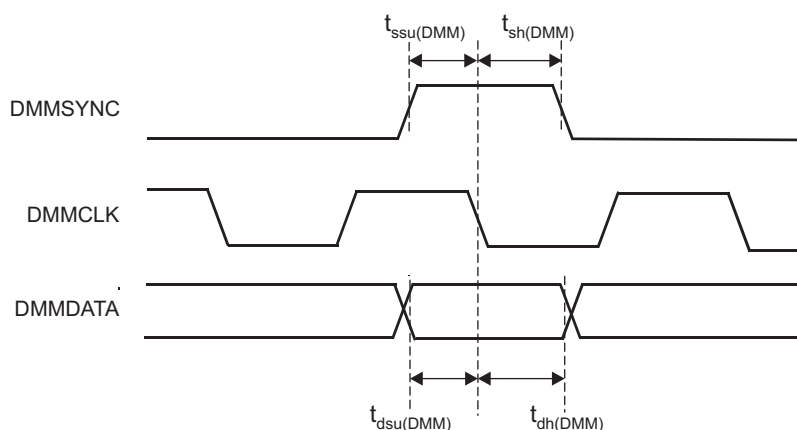
Figure 5-18. DMMDATA Timing
