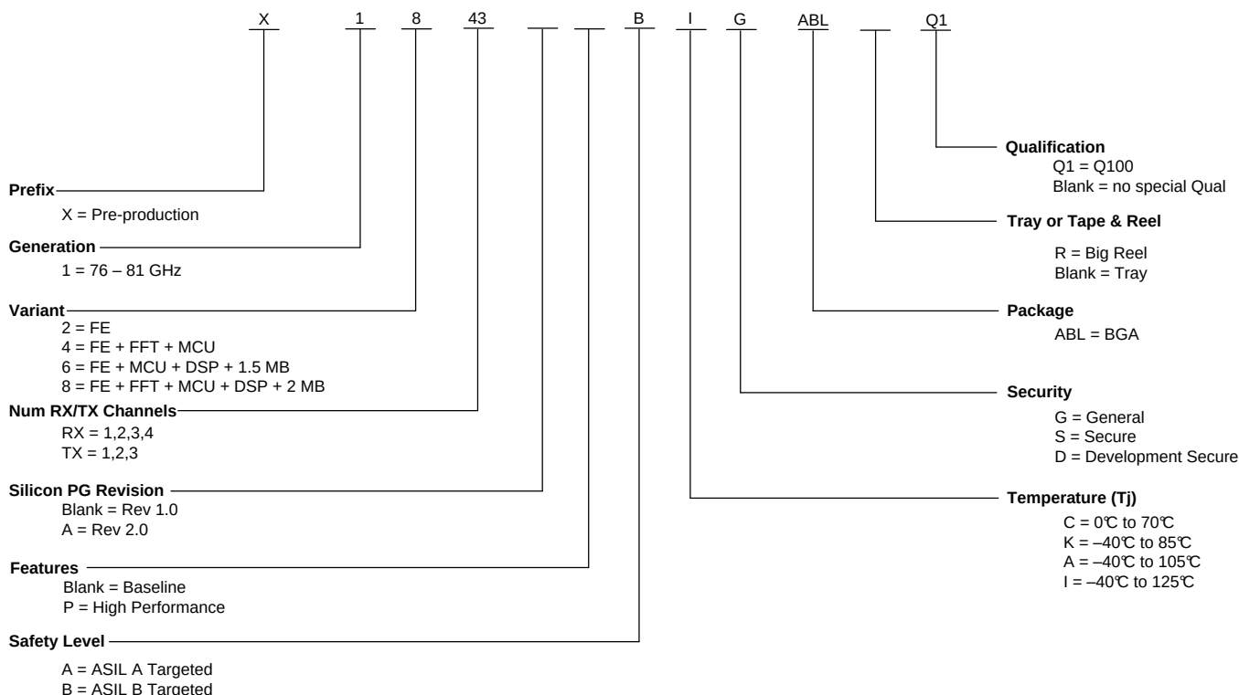
Figure 9-1. Device Nomenclature
