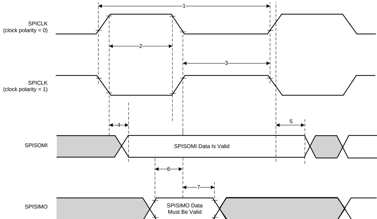
Figure 5-7. SPI Slave Mode External Timing (CLOCK PHASE = 0)
