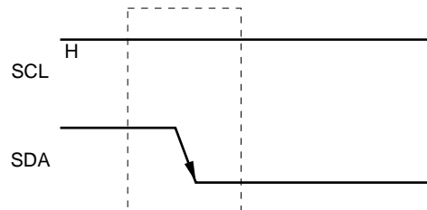
Figure 16-41. Start Condition
