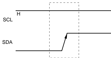
Figure 16-45. Stop Condition
