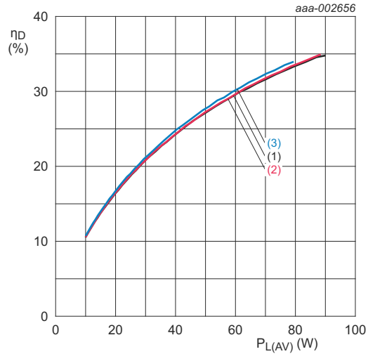
V_{DS} = 32\text{ V}; I_{Dq} = 1700\text{ mA}. (1) f = 2600\text{ MHz} (2) f = 2650\text{ MHz} (3) f = 2700\text{ MHz}
