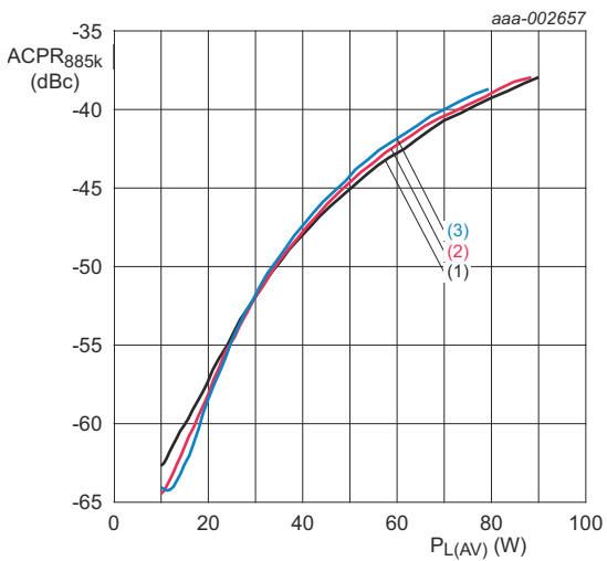
V_{DS} = 32\text{ V}; I_{Dq} = 1700\text{ mA}. (1) f = 2600\text{ MHz} (2) f = 2650\text{ MHz} (3) f = 2700\text{ MHz}
