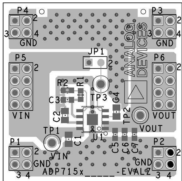
Figure 2. ADP7159RD-04-EVALZ (8-Lead SOIC) PCB Layout
