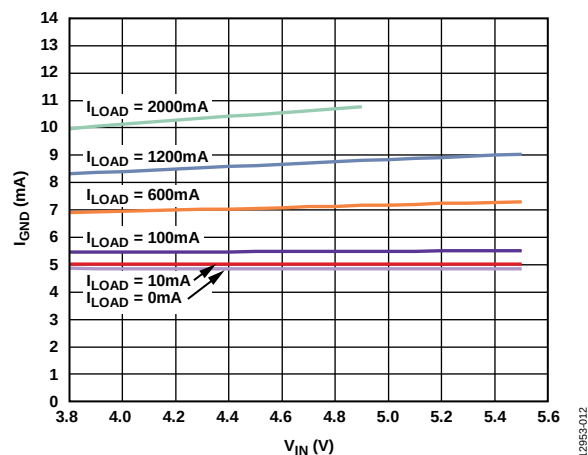
Figure 12. Ground Current ( I_{GND} ) vs. Input Voltage ( V_{IN} ), V_{OUT} = 3.3\text{ V} , T_A = 25^\circ\text{C} , C_{IN} = C_{OUT} = 10\text{ }\mu\text{F}
