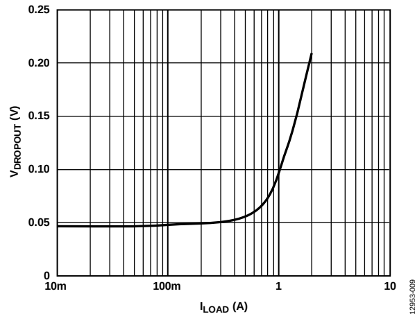
Figure 9. Dropout Voltage vs. Load Current ( I_{LOAD} ), V_{OUT} = 3.3 V, T_A = 25^\circ\text{C} , C_{IN} = C_{OUT} = 10\ \mu\text{F}
