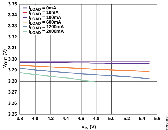
Figure 7. Output Voltage ( V_{OUT} ) vs. Input Voltage ( V_{IN} ), V_{OUT} = 3.3 V, T_A = 25^\circ\text{C} , C_{IN} = C_{OUT} = 10\ \mu\text{F}
