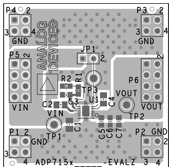
Figure 1. ADP7159CP-04-EVALZ (10-Lead LFCSP) Printed Circuit Board (PCB) Layout
