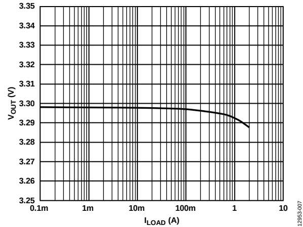
Figure 8. Output Voltage ( V_{OUT} ) vs. Load Current ( I_{LOAD} ), V_{OUT} = 3.3 V, T_A = 25^\circ\text{C} , C_{IN} = C_{OUT} = 10\ \mu\text{F}
