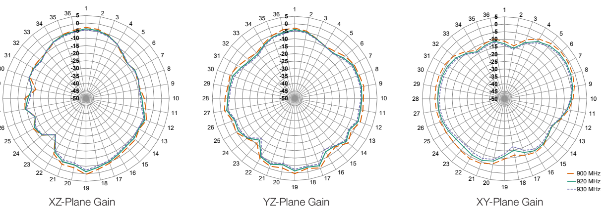
Figure 7. ANT-8/9-HDP-2000-ccc Radiation Patterns
