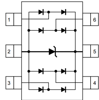
Schematic And Pinning Diagram
