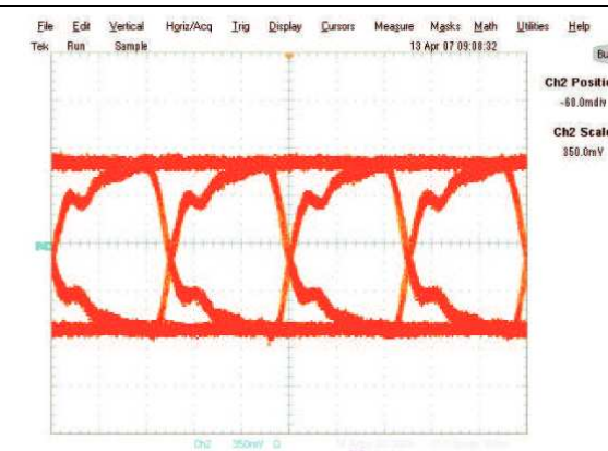
Figure 27. Typical Eye Pattern SN65LVDS180: Tx + Rx
