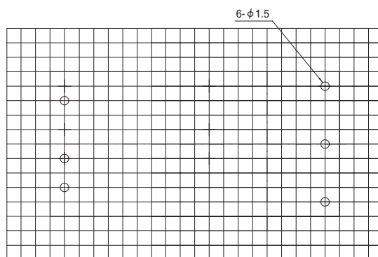
※Recommended Pad and Hole dia. (TOP VIEW)
