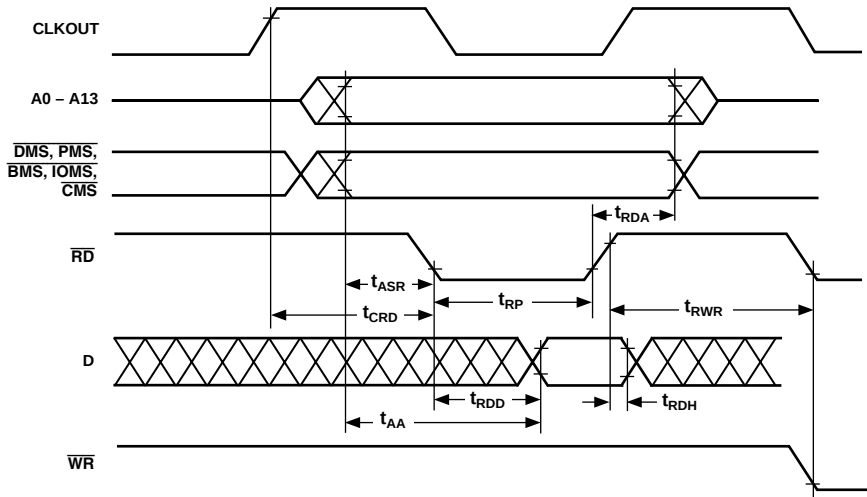
Figure 12. Memory Read
