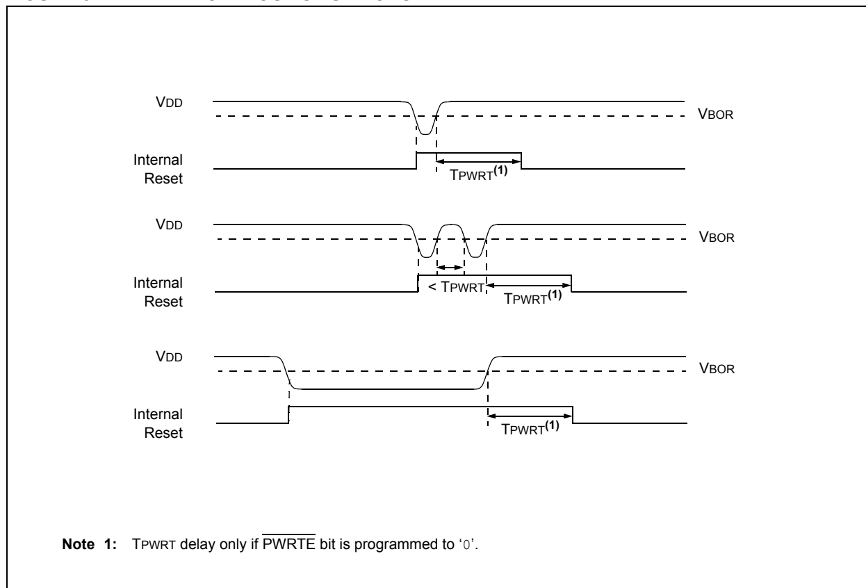
FIGURE 5-2: BROWN-OUT SITUATIONS
