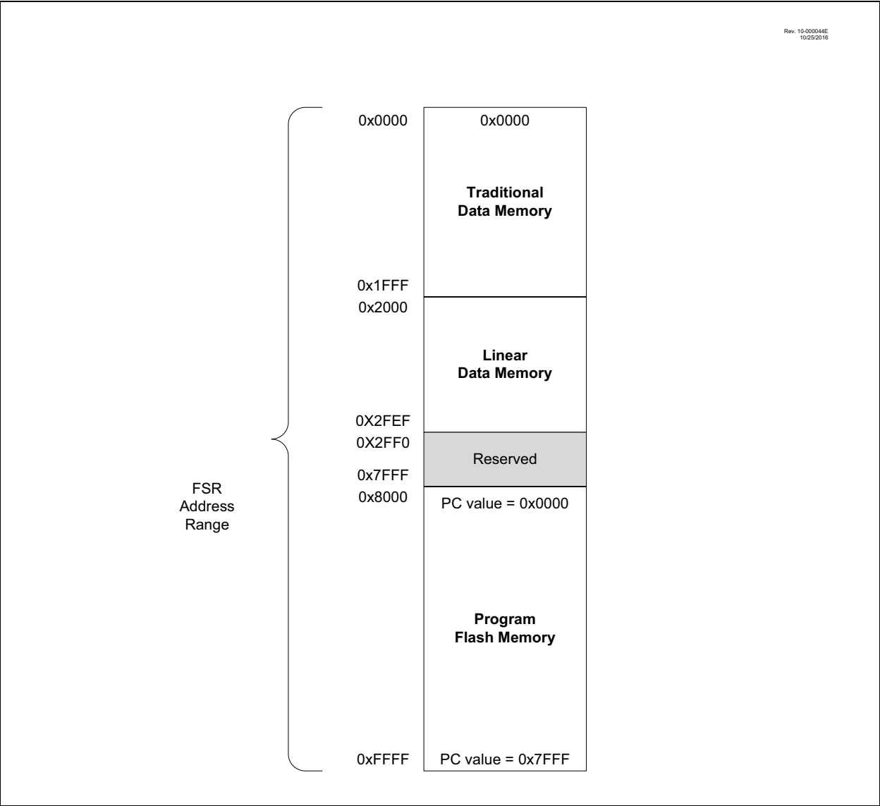
FIGURE 3-8: INDIRECT ADDRESSING
