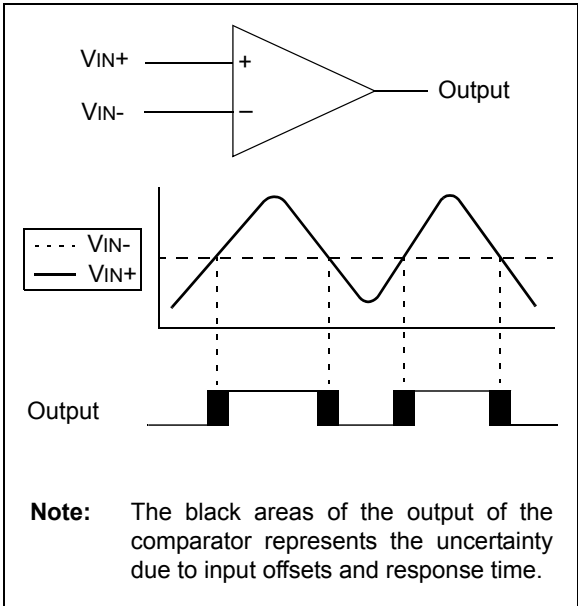
FIGURE 18-1: SINGLE COMPARATOR
