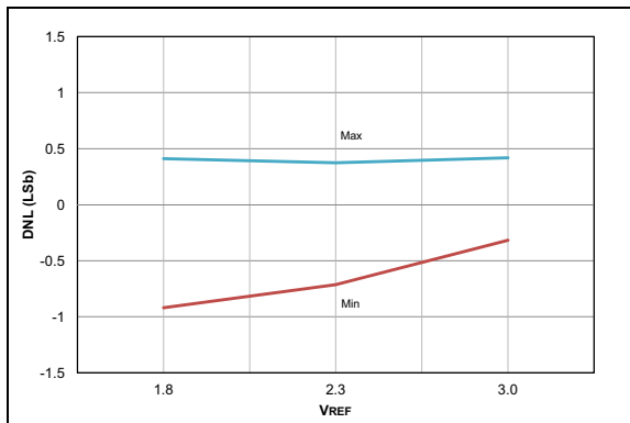
FIGURE 38-39: ADC 10-bit Mode, Single-Ended DNL, V_{DD} = 3.0V , T_{AD} = 1\text{ }\mu s .
