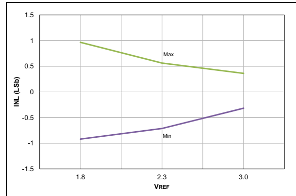
FIGURE 38-40: ADC 10-bit Mode, Single-Ended INL, V_{DD} = 3.0V , T_{AD} = 1\text{ }\mu s .
