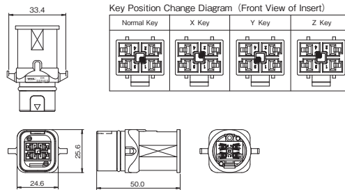
Receptacle Housing
