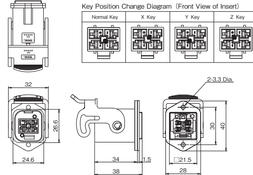
Receptacle Housing
