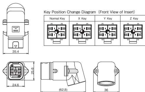
Tab Housing
