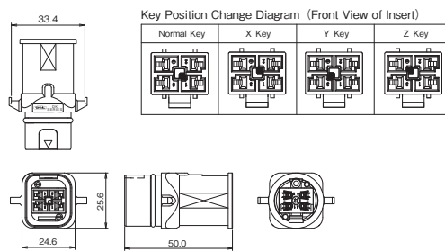
Receptacle Housing
