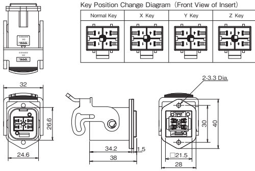
Tab Housing
