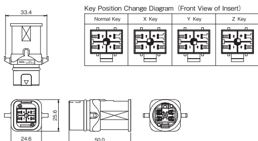
Tab Housing
