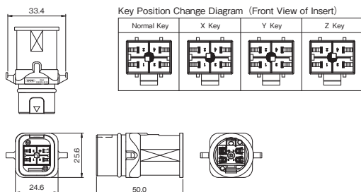
Tab Housing
