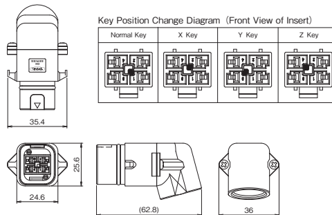
Receptacle Housing
