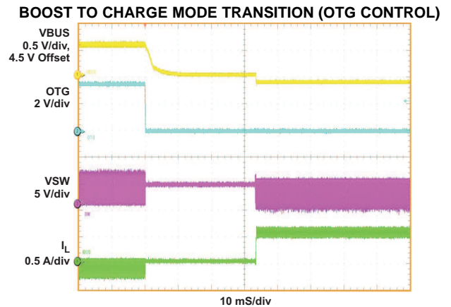
Figure 18. V_{BUS} = 4.5\text{ V} (Charge Mode) / 5.1\text{ V} (Boost Mode), V_{BAT} = 3.5\text{ V} , I_{IN\_LIM} = 500\text{ mA} , (32S mode)
