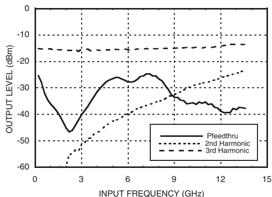
Output Harmonic
