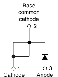
TO-247AC modified
