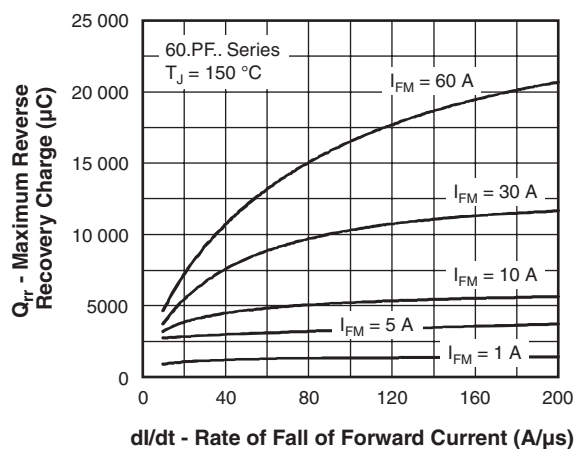
Fig. 11 - Recovery Charge Characteristics, T_J = 150\text{ }^{\circ}\text{C}
