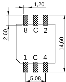
RECOMMENDED LAYOUT
